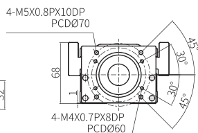
View B
